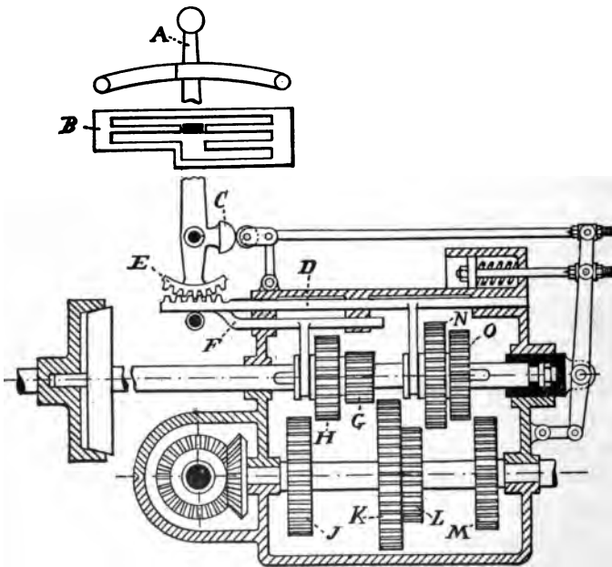
FIG. 256 --Transmission Gear of the Cannstadt-Daimler Carriage shown in the last figure. Here, A is the hand lever; B, the gridiron quadrant; C, a dog on the lever for throwing out the clutch in shifting the gears; E, toothed sector at end of A for actuating rack rods D and F (see next figure); G and H, low speed gears on the clutch shaft; J and K, low-speed gears on the second, or driving, shaft; N and O, high-speed gears on the clutch shaft; L and M, high-speed gears on the second shaft. H and G are shifted on square portion of shaft by rack, F; N and O by rack, D.
